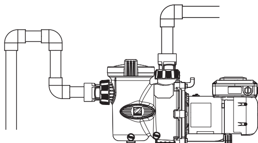
FIGURE 3 - INSTALLATION INCORRECTE
