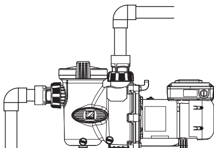
FIGURE 2 - INSTALLATION CORRECTE
