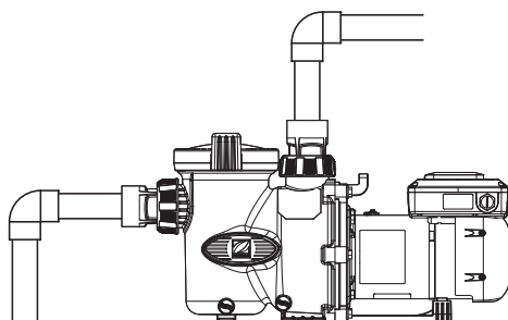
FIGURE 2 - INSTALLATION CORRECTE
